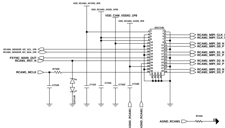
RCAM1_50M(30PIN) A14 5G BASE
