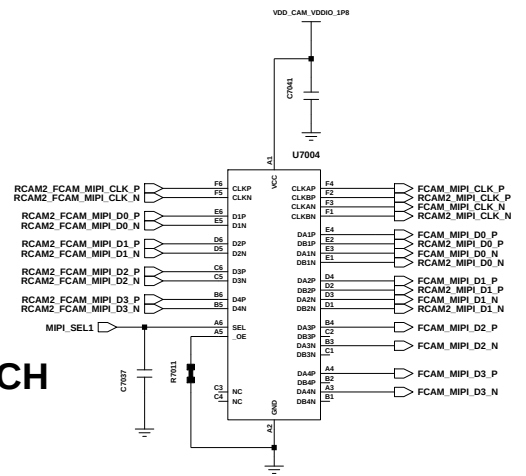
FRONT_13M CAMERA (24PIN) A14 5G BASE
