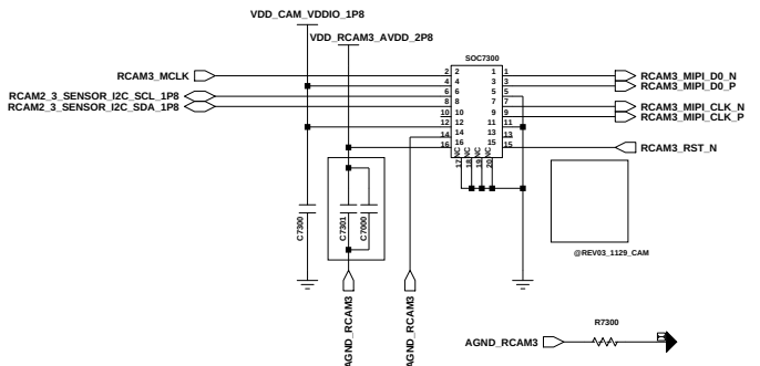
RCAM3_2M MACRO CAMERA(16PIN) A14 5G BASE
